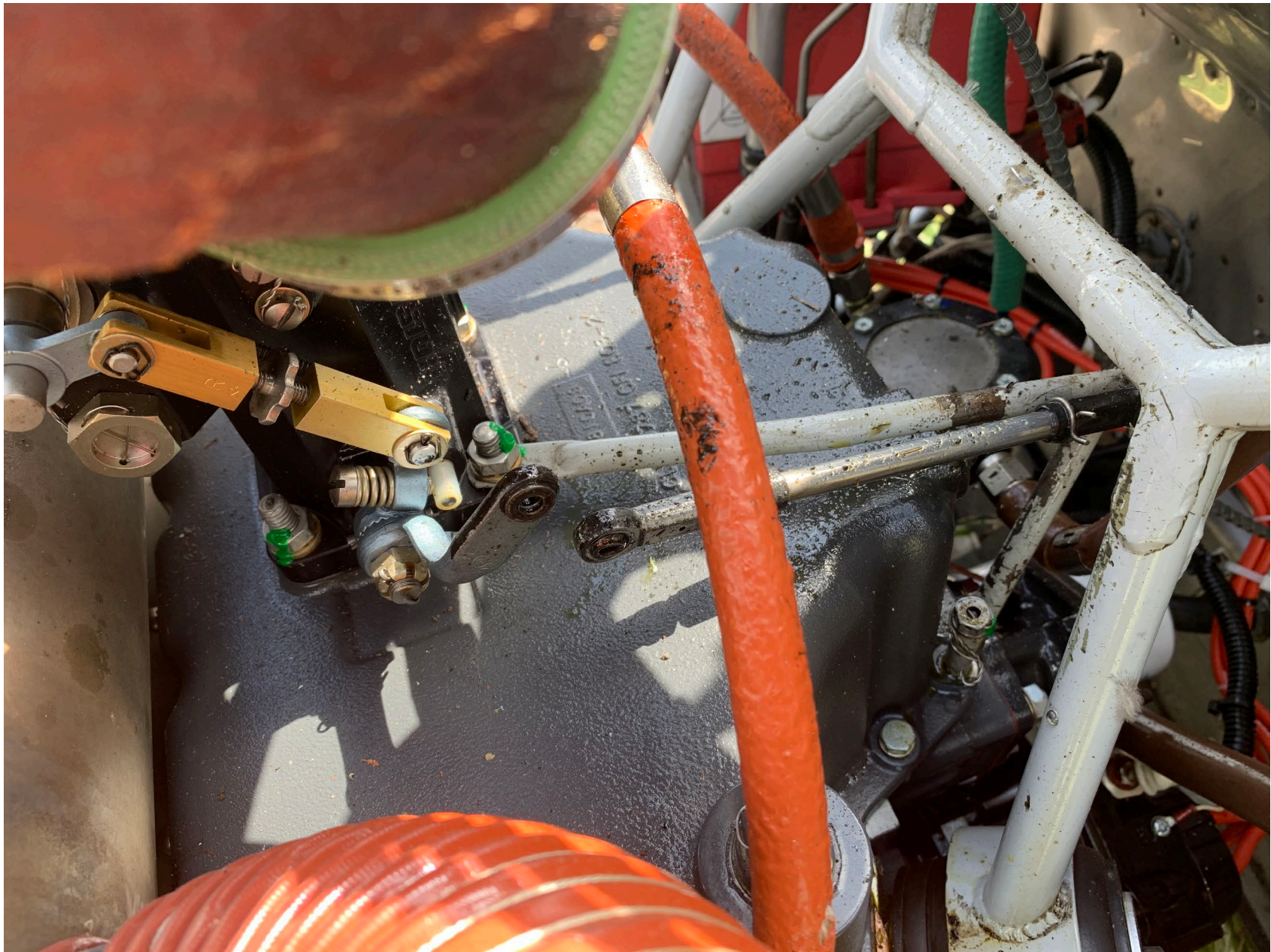
Photo 5 – Throttle Cable/Fuel Injector Servo Linkage (FAA Photo)
