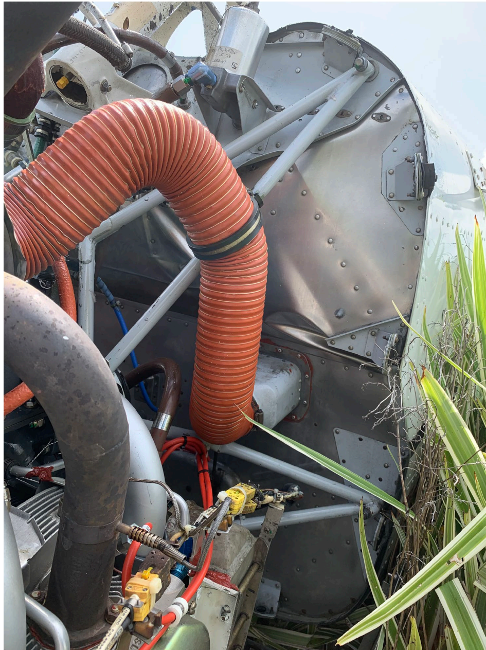
Photo 4 – Engine Firewall Damage (FAA Photo)
