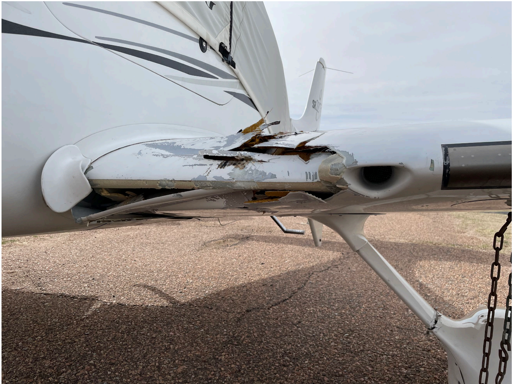
Photo 1 – Left Wing Damage
