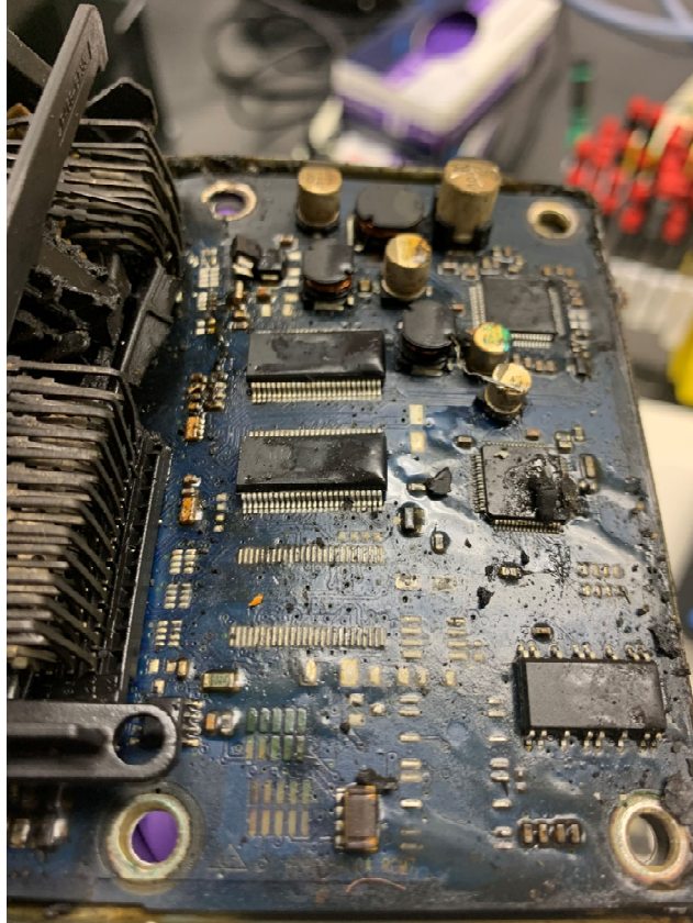
Photograph 3: The damaged ACM chip board
