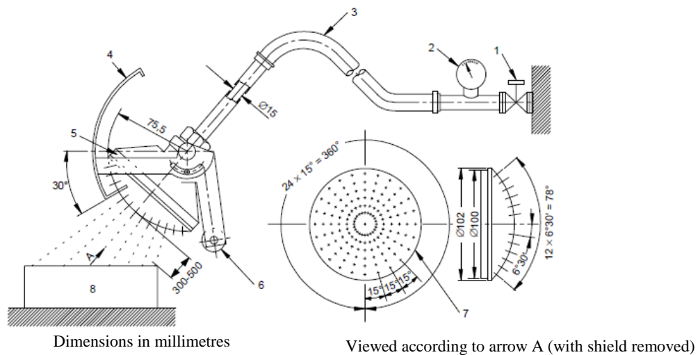
Figure 2 Splashing test nozzle
