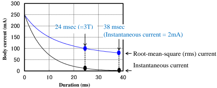
Figure 8 Body Current for 0.2 J and 200 V Capacitor under Large Area Hand-to-Hand Contact Under Wet Conditions (800 Ω Body Resistance)
