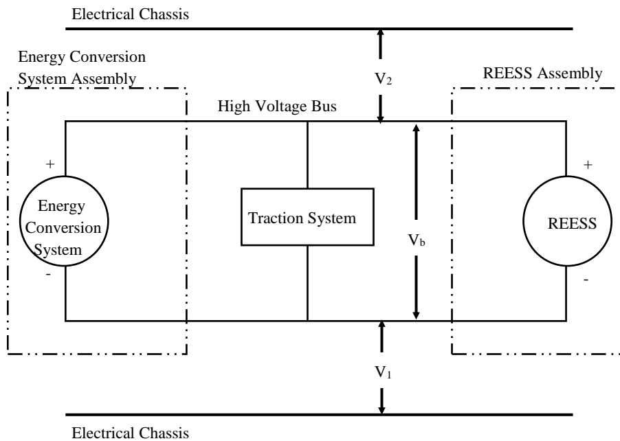
Figure 7 Measurement of V_b , V_1 , V_2
