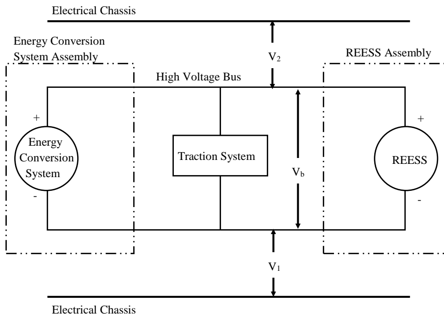
Figure 18 Measurement of V_b , V_1 , V_2
