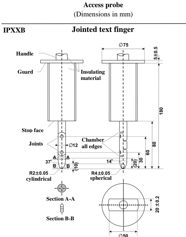
Figure 5 Jointed Test Finger
