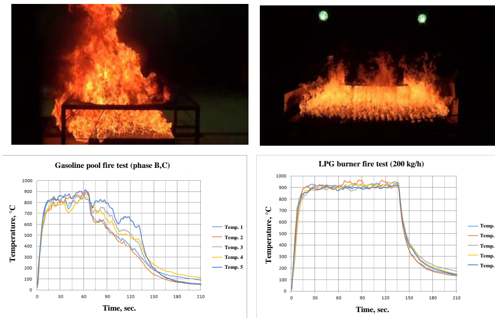
Figure 22 Test scene photographs and temperature measurements of a gasoline pool fire and an LPG burner fire
