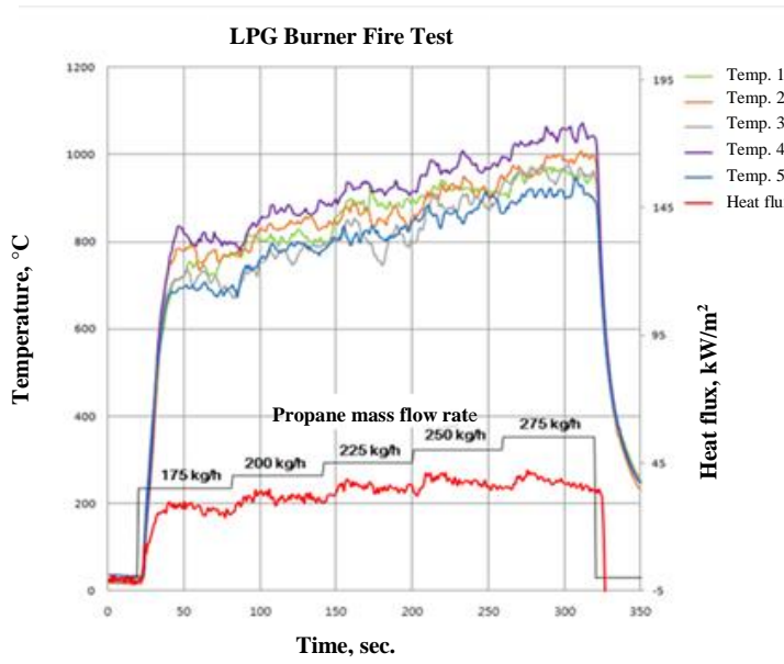
Figure 20 Flame temperature and heat flux of an LPG burner fire with increasing LPG mass flow rate (without Tested-Device)
