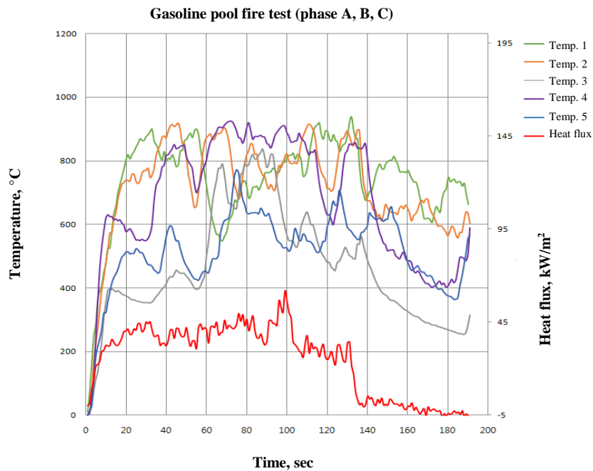
Figure 21 Flame temperature and heat flux of gasoline pool fire (without Tested-Device)
