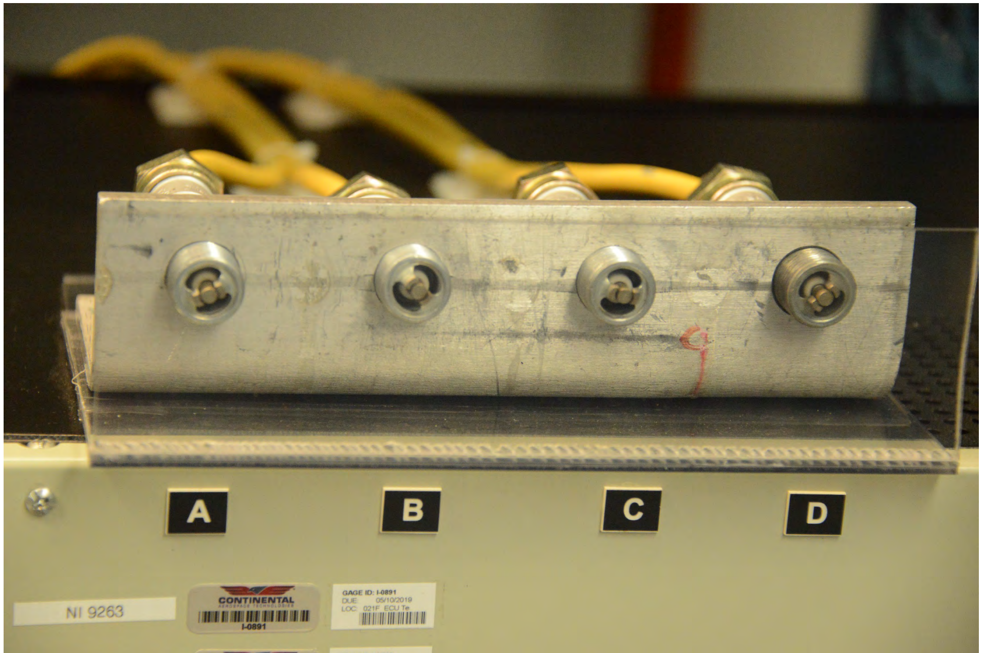
Photo 7 - View of sparkplugs attached to the accident FADEC MPC.
