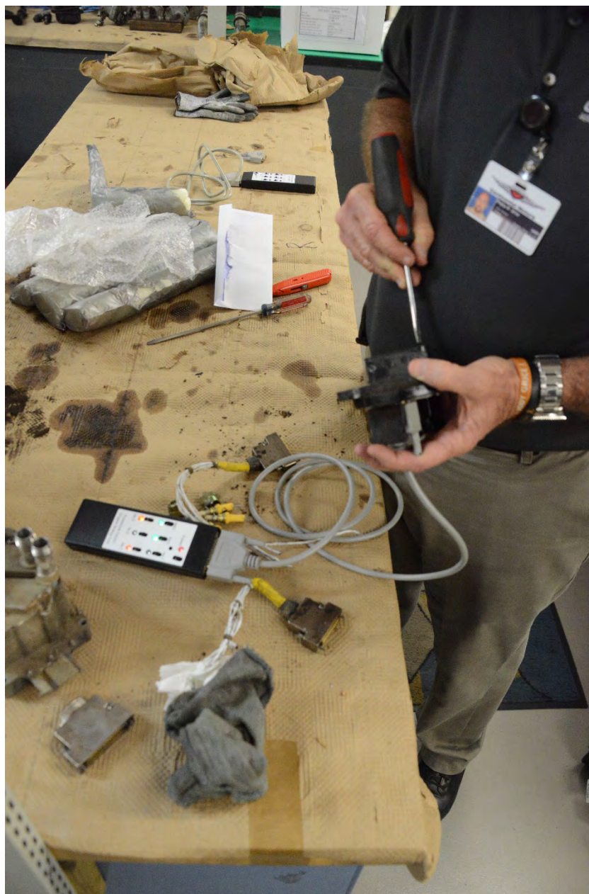
Photo 9 - View of the speed sensor connected to a testing system.
