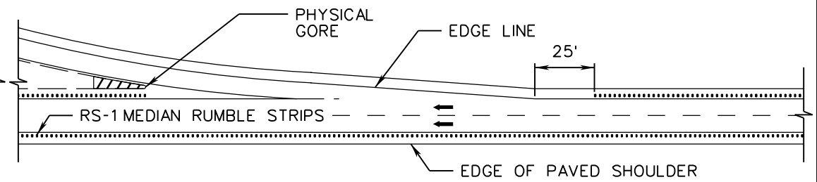
PLAN VIEW
