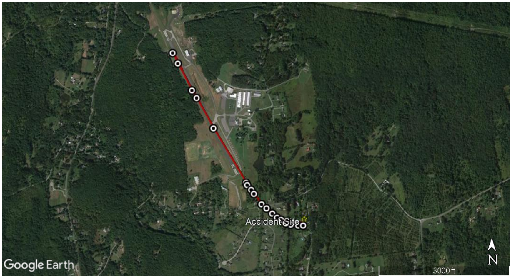
Figure 1 ADS-B Data – Overall
