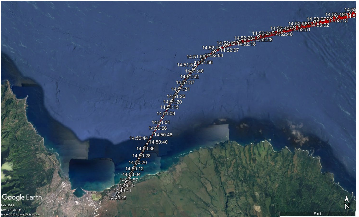
Figure 2 ADS-B Flight Track - Overhead View
