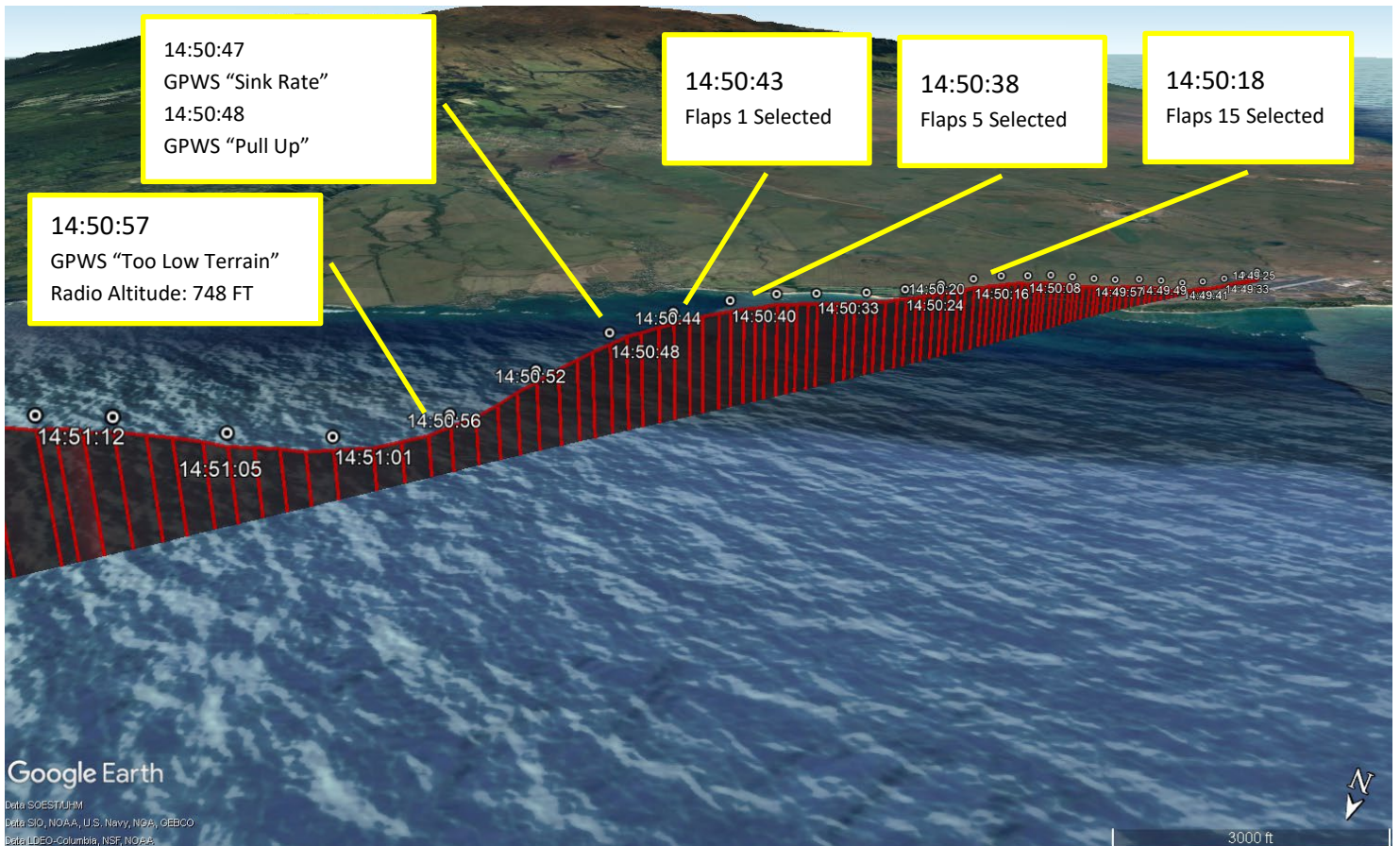
Figure 1 - ADS-B Flight Track - Perspective View
