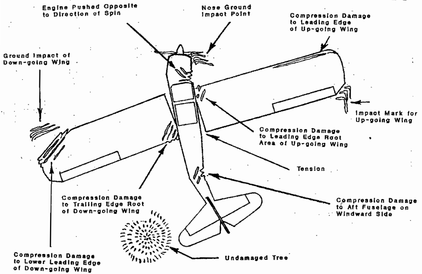
Figure 27-17. Wreckage Pattern of a Spinning Airplane
