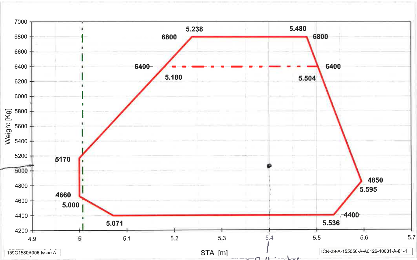
Figure 1-1 Weight and Longitudinal CG Limitations
