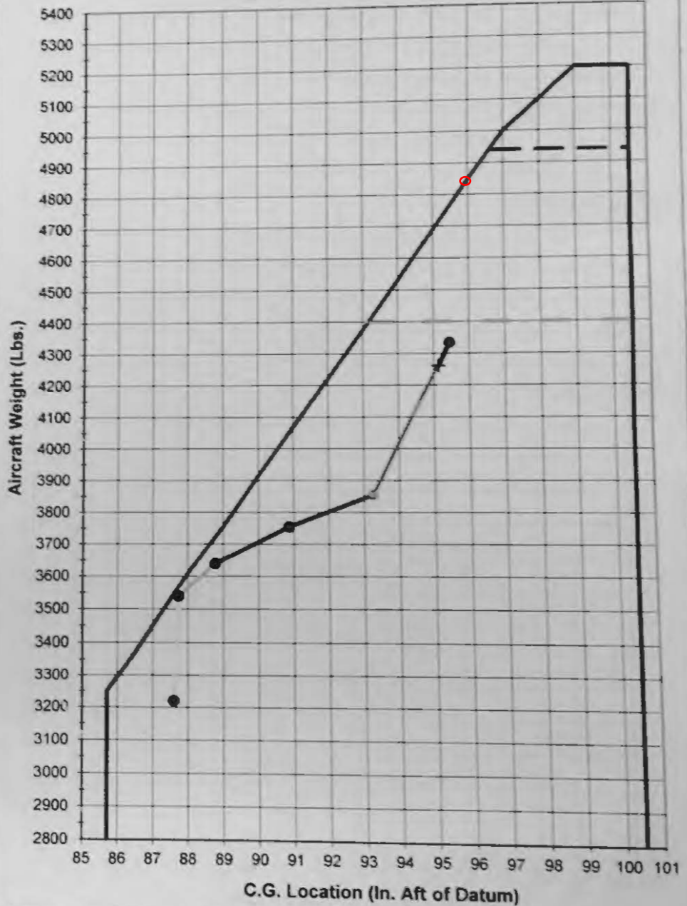
Weight & Balance Graph
