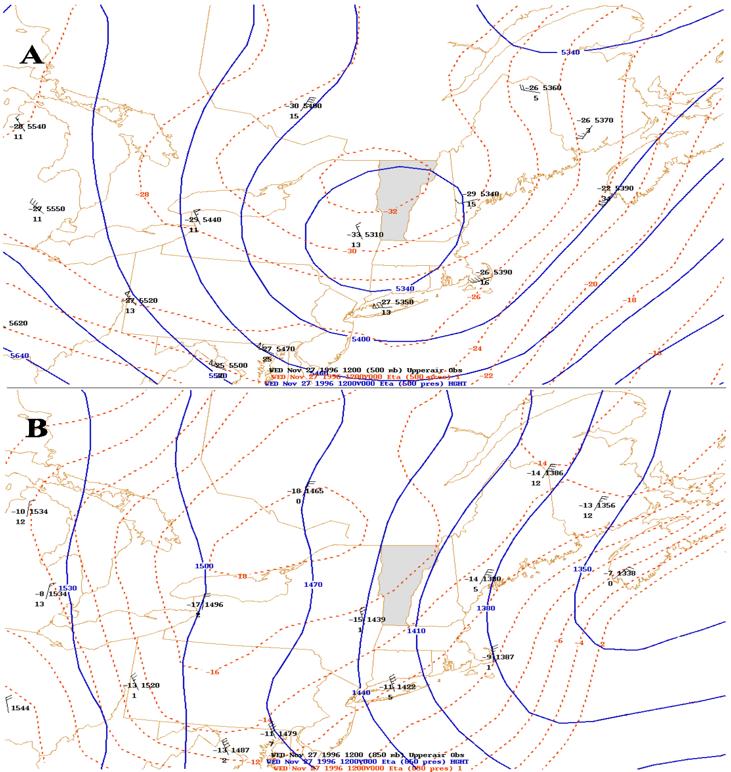
Figure 6. Upper air analyses from the Eta model on 27 November 1996 at 1200 UTC showing a 500-mb closed low (A) and 850-mb cold air advection (B). Solid lines are geopotential heights drawn every 60-m (A) and 30-m (B). Dashed lines are isotherms contoured every 2°C.
