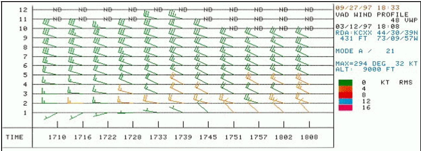
Figure 15. Same as Fig. 3, expect it is for 12 March 1997 between 1710 to 1808 UTC. It shows the passage of a surface trough around 1730 UTC.
