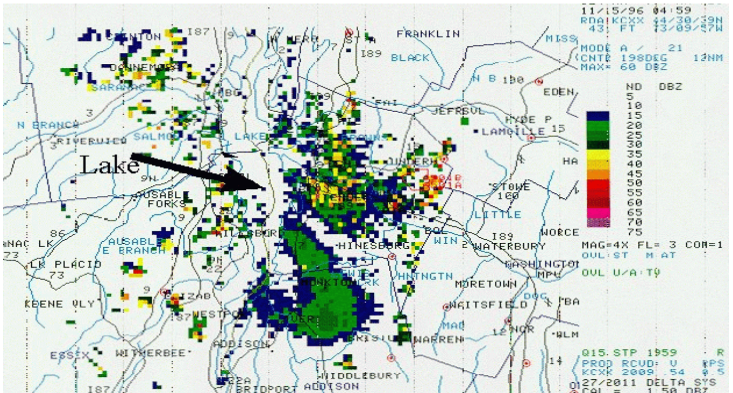
Figure 11. KCXX composite reflectivity image at 0459 UTC 15 November 1996. A band of lake effect snow extending from the southern end of Lake Champlain produced a steady snowfall from 0100 to 1000 UTC on 15 November 1996. The color table on the right depicts the intervals of maximum reflectivity in units of dBZ.
