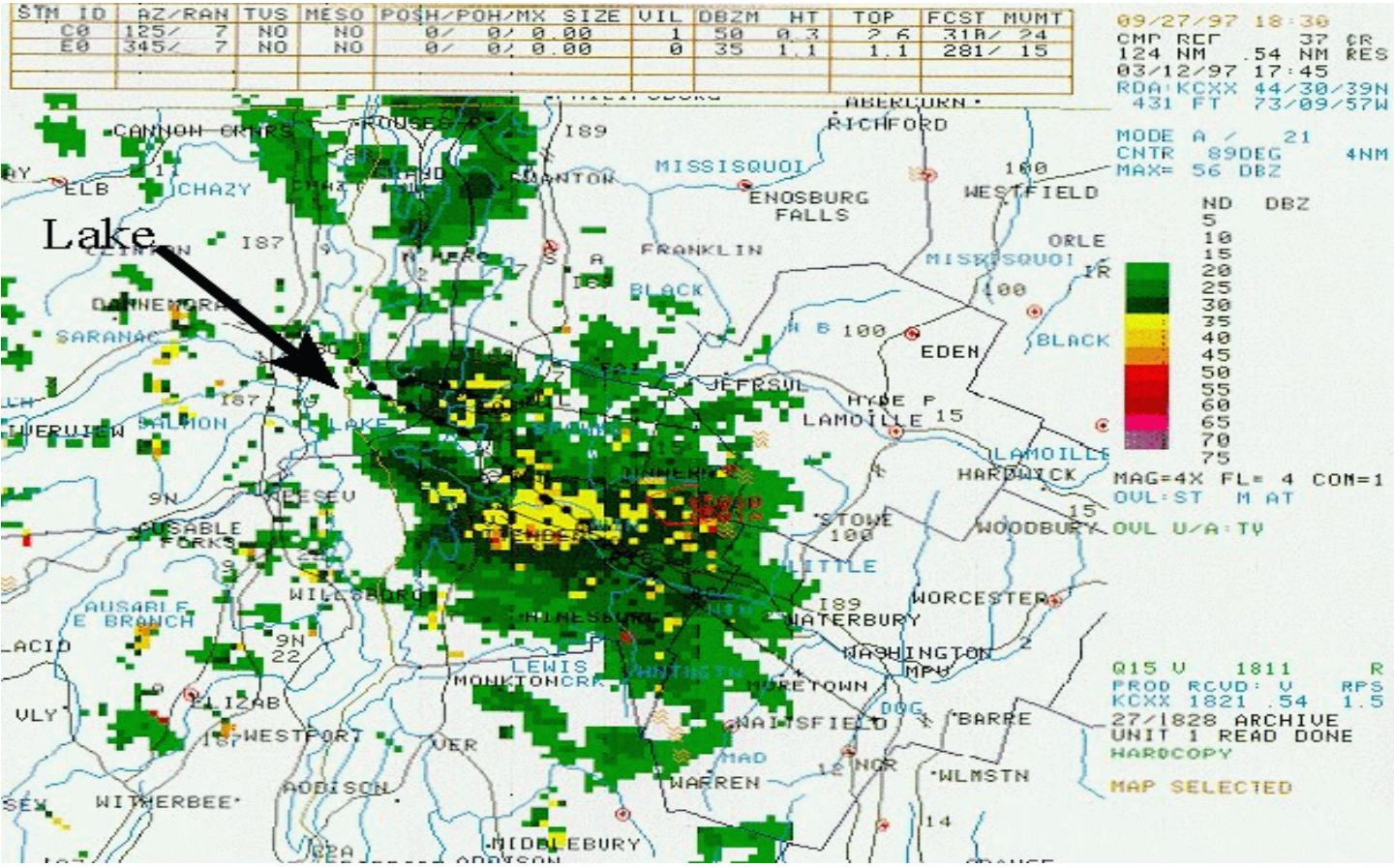
Figure 16. An example of lake enhanced snow squalls depicted by KCXX composite reflectivity at 1745 UTC on 12 March 1997. Burlington is located in the large area of 35-39 dBZ which was producing heavy snow. Other light snow showers are seen on the windward side of Lake Champlain. The WSR-88D SCIT algorithm identified this cell (black dots and line) and tracked it across the lake. The color table on the right depicts the intervals of maximum reflectivity in units of dBZ.
