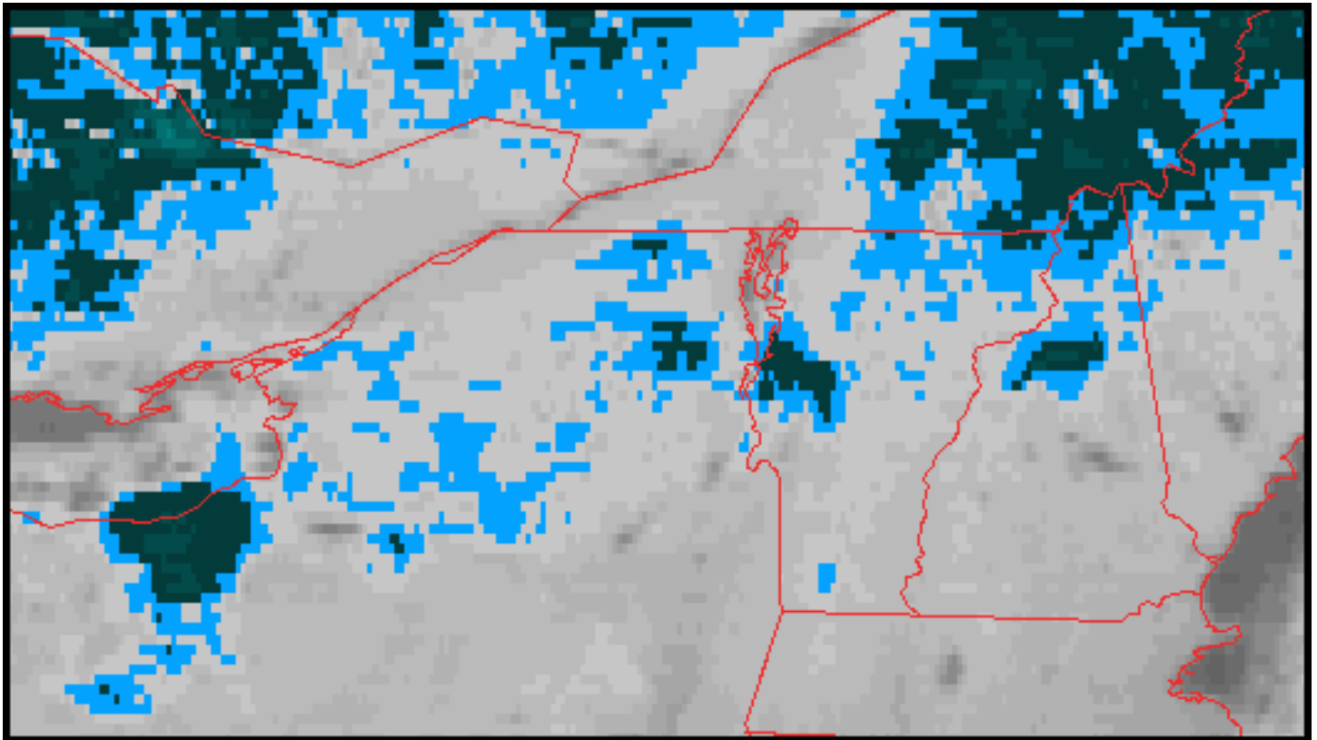
Figure 12. GOES-8 10.7 \mu\text{m} satellite image at 0915 UTC on 15 November 1996 showing a band of lake effect enhanced cold cloud tops ( -18^{\circ}\text{C} is the dark blue) extending southeast of Lake Champlain.
