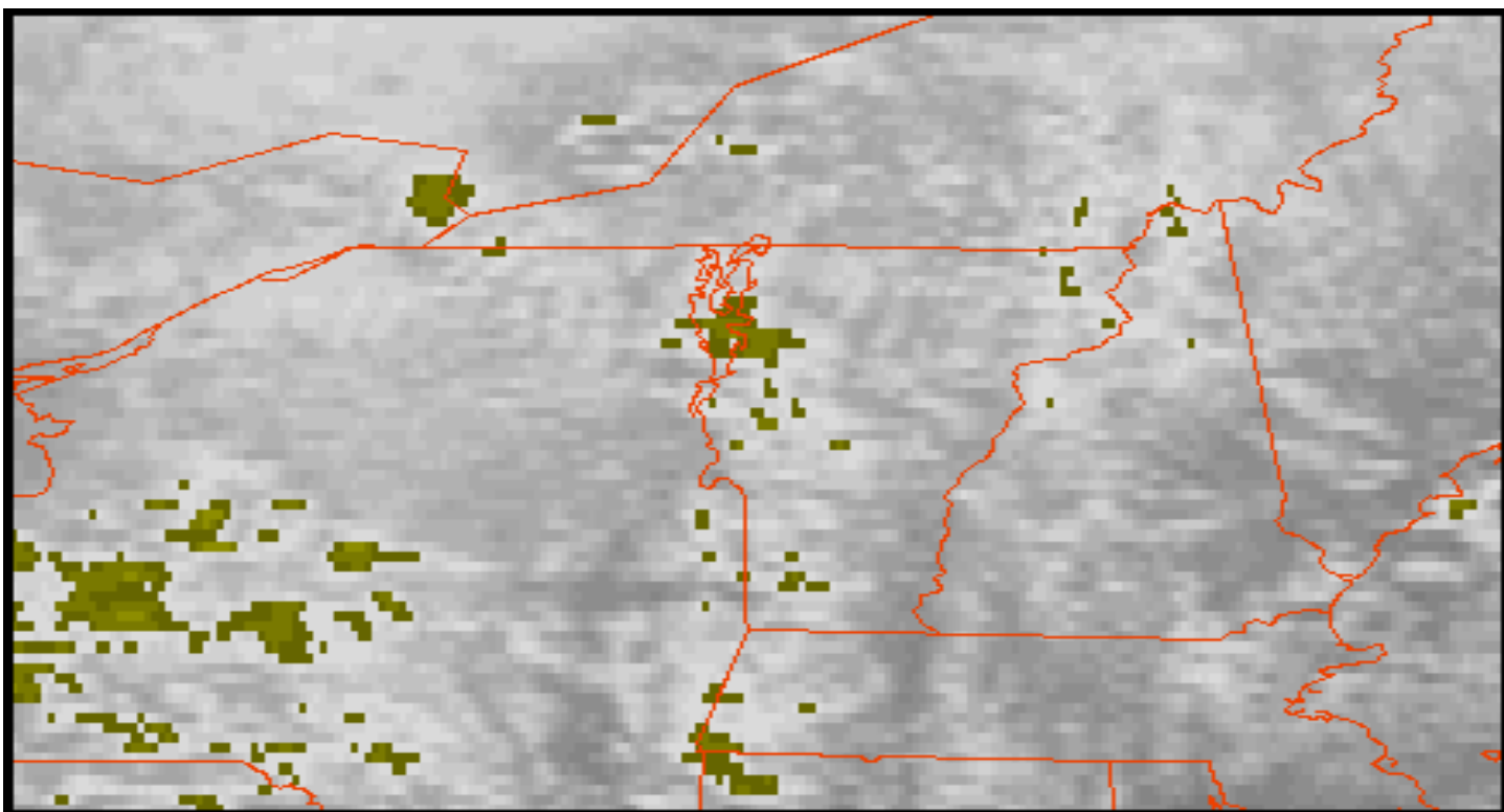
Figure 22. GOES-8 10.7 \mu\text{m} satellite image taken at 1745 UTC on 12 November 1996 depicting one of the heavy snow squalls that affected Burlington. Cloud top temperatures over Lake Champlain were between -20 and -25 ^{\circ}\text{C} indicated by the greenish-yellow enhancement.
