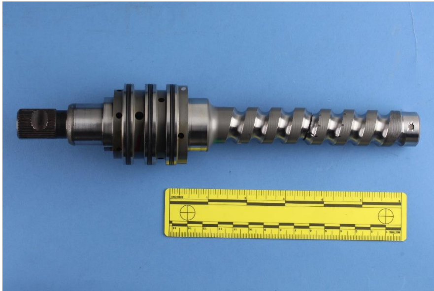
Photo 5 – Internal helical worm gear from the steering gearbox of the 2015 IC school bus
