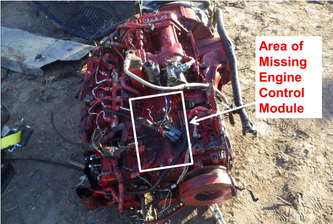
Photo 8 - View of detached bus engine showing area of missing engine control module from the 2015 Blue Bird Vision bus modified for prison transport.
