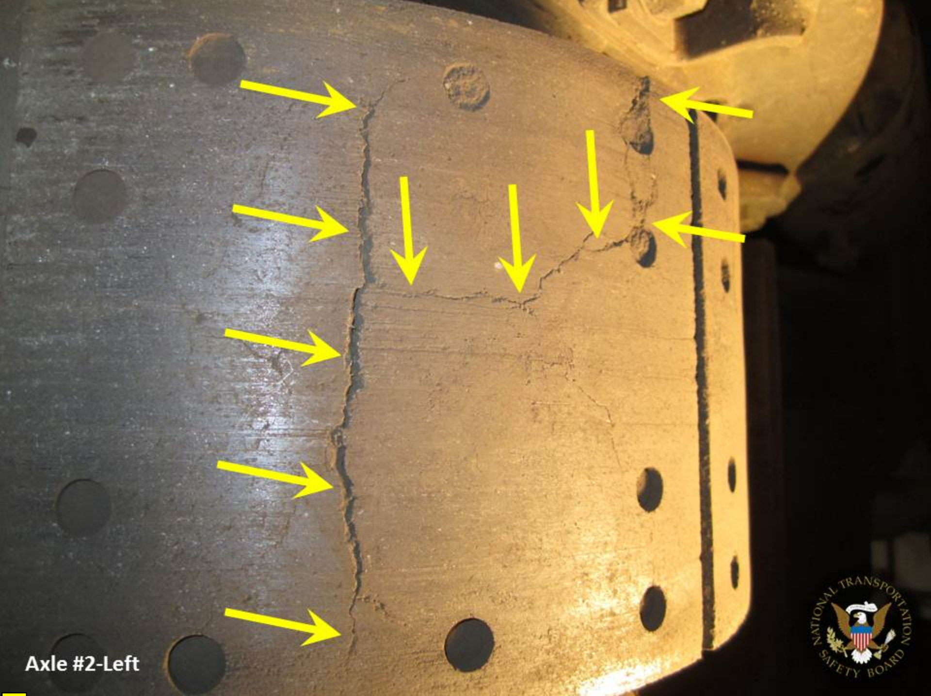
Photo 12 – 2004 Mack Truck – Cracks in Lower Rear Brake Pad on Left Side of Axle #2
