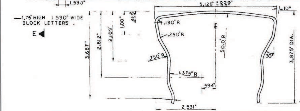
SECTION E-E SCALE: FULL SIZE MATERIAL THICKNESS 0.09" MIN.
