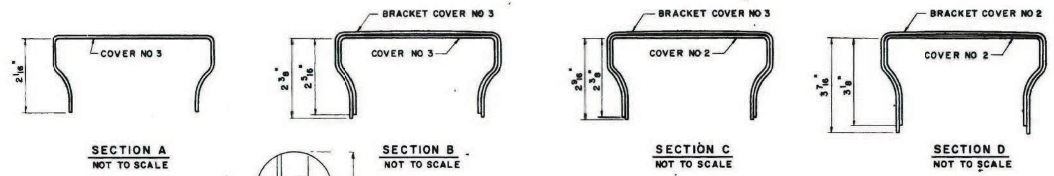
END APPROACH COVERS NOT TO SCALE
