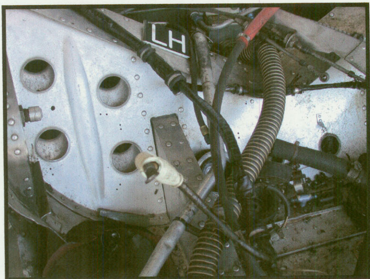
BAUK-224 Left engine nacelle
