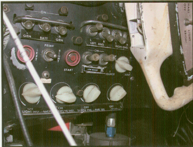
BAUK-218 Fuel boost pump switches in panel
