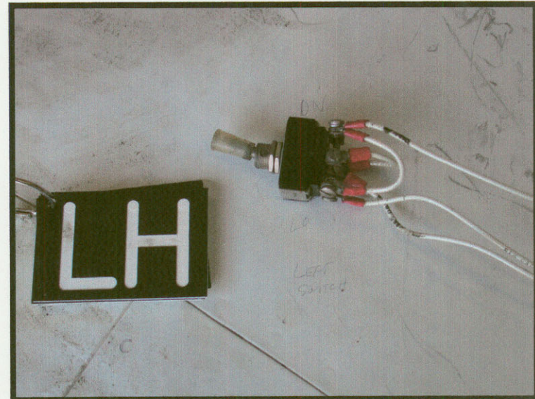
BAUK-219 Left fuel boost pump switch
