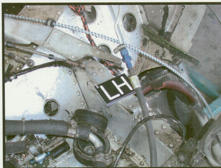
BAUK-225 Left engine nacelle
