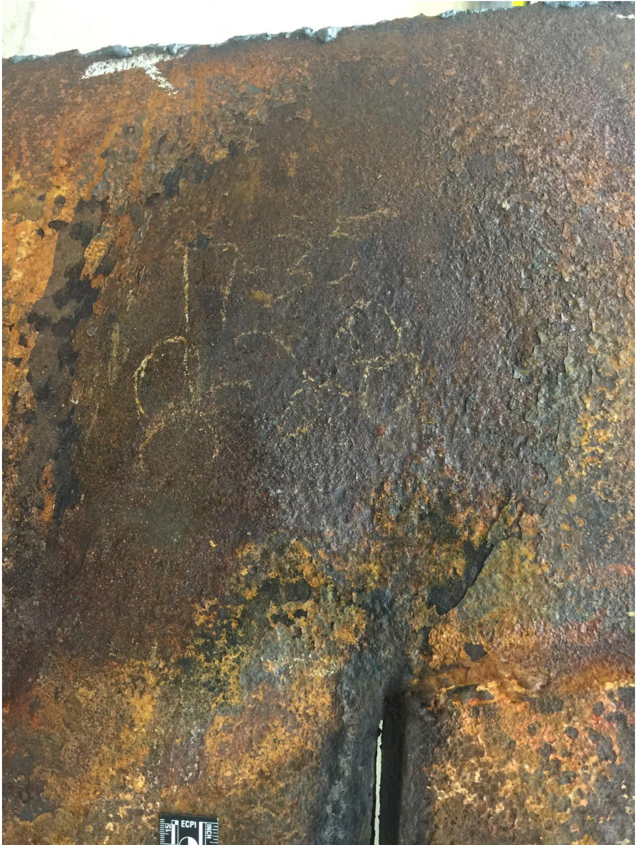
Tank shell scaling exterior surface, right side of A-end inboard cradle pad termination.
