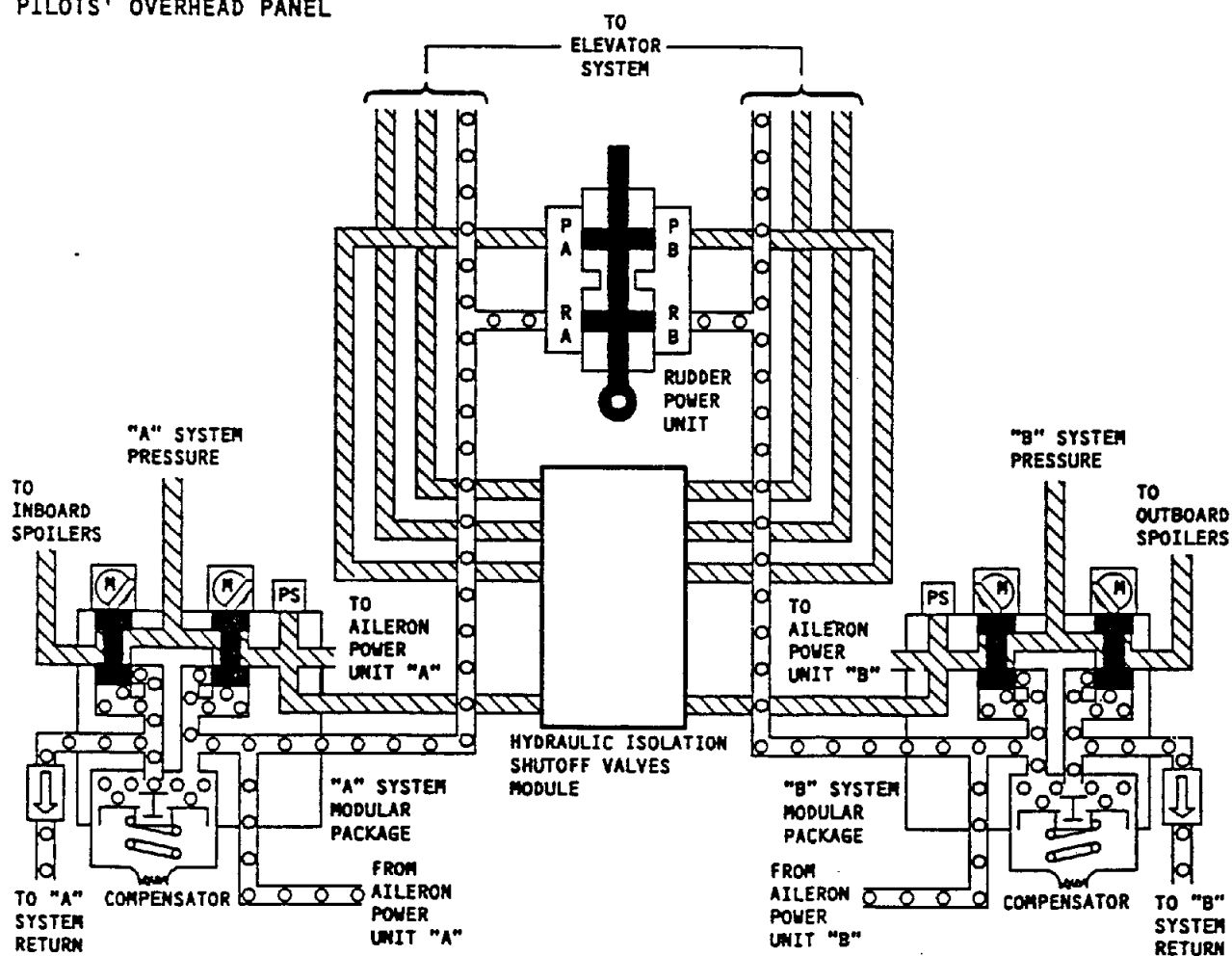
PILOTS' OVERHEAD PANEL
