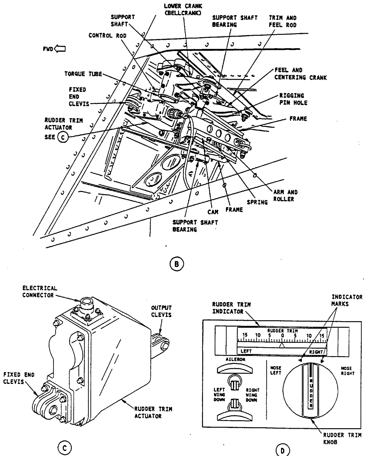
Rudder Trim and Feel System Figure 4 (Sheet 2)
