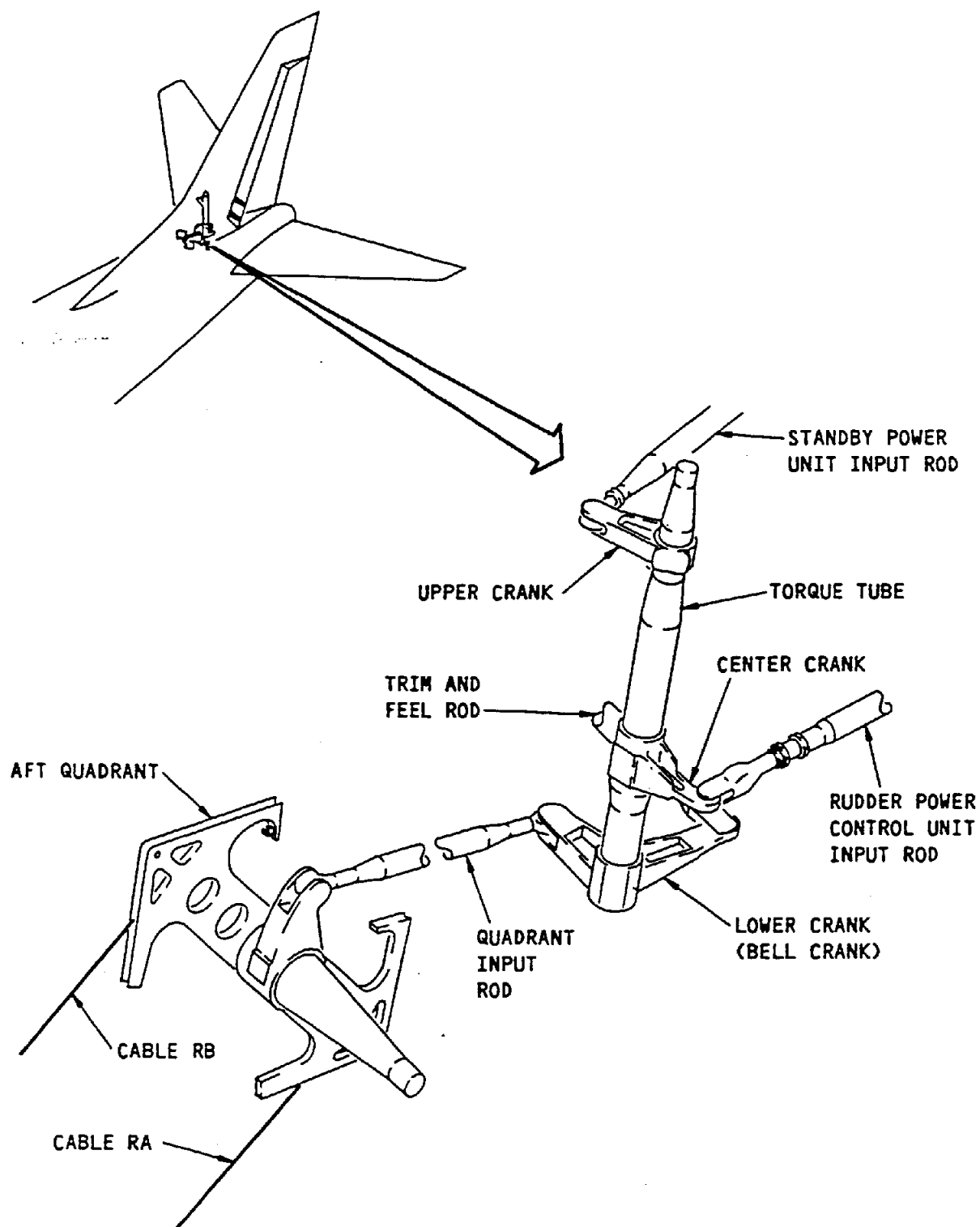
AFT RUDDER CONTROL COMPONENT
