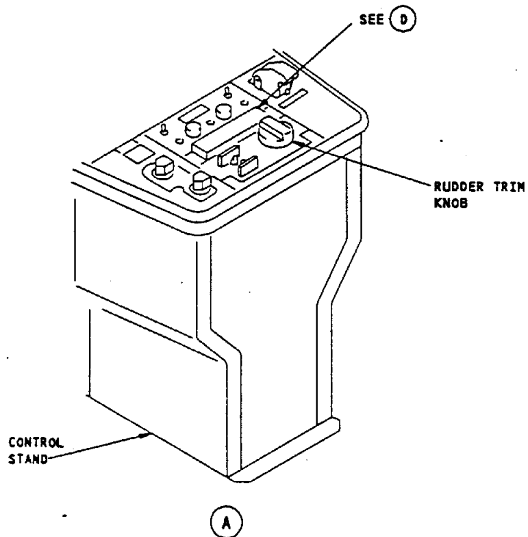
Rudder Trim and Feel System Figure 4 (Sheet 1)
