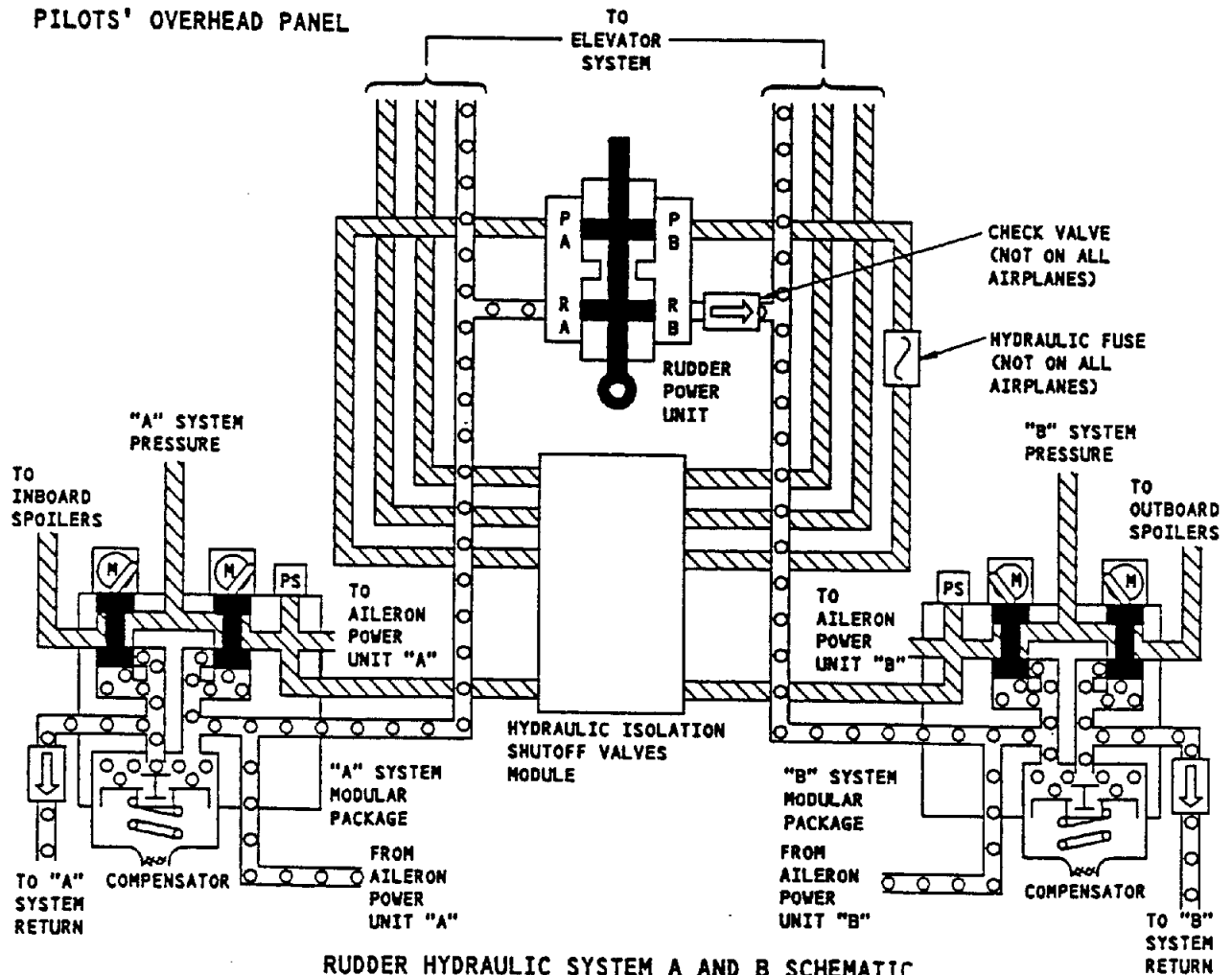
Rudder Hydraulic System Schematic
