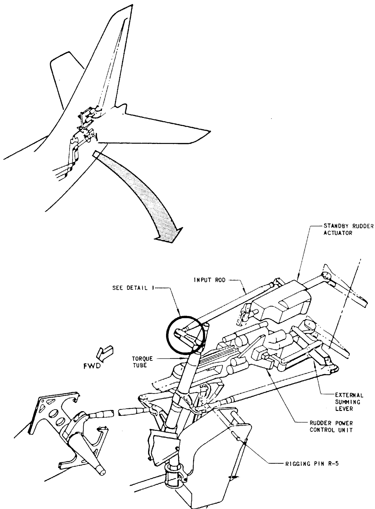
FIGURE 1. RUDDER AUXILIARY POWER CONTROL UNIT SHEAR PIN REPLACEMENT
