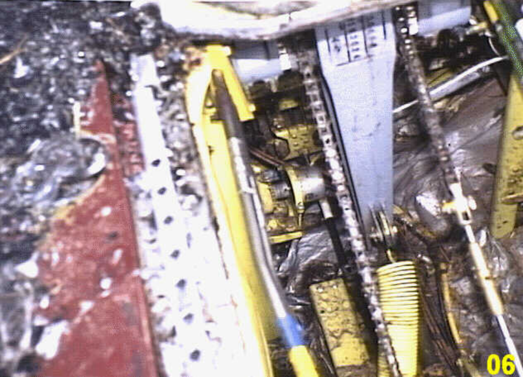
Systems 9A - Photo 06. View of FDR rudder pedal potentiometer installation
