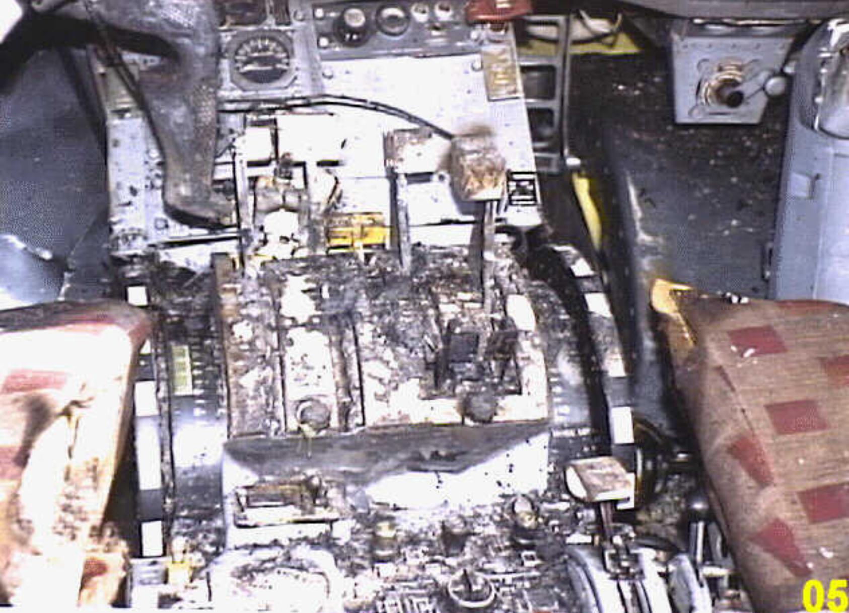
Systems 9A - Photo 05. Throttle Quadrant
