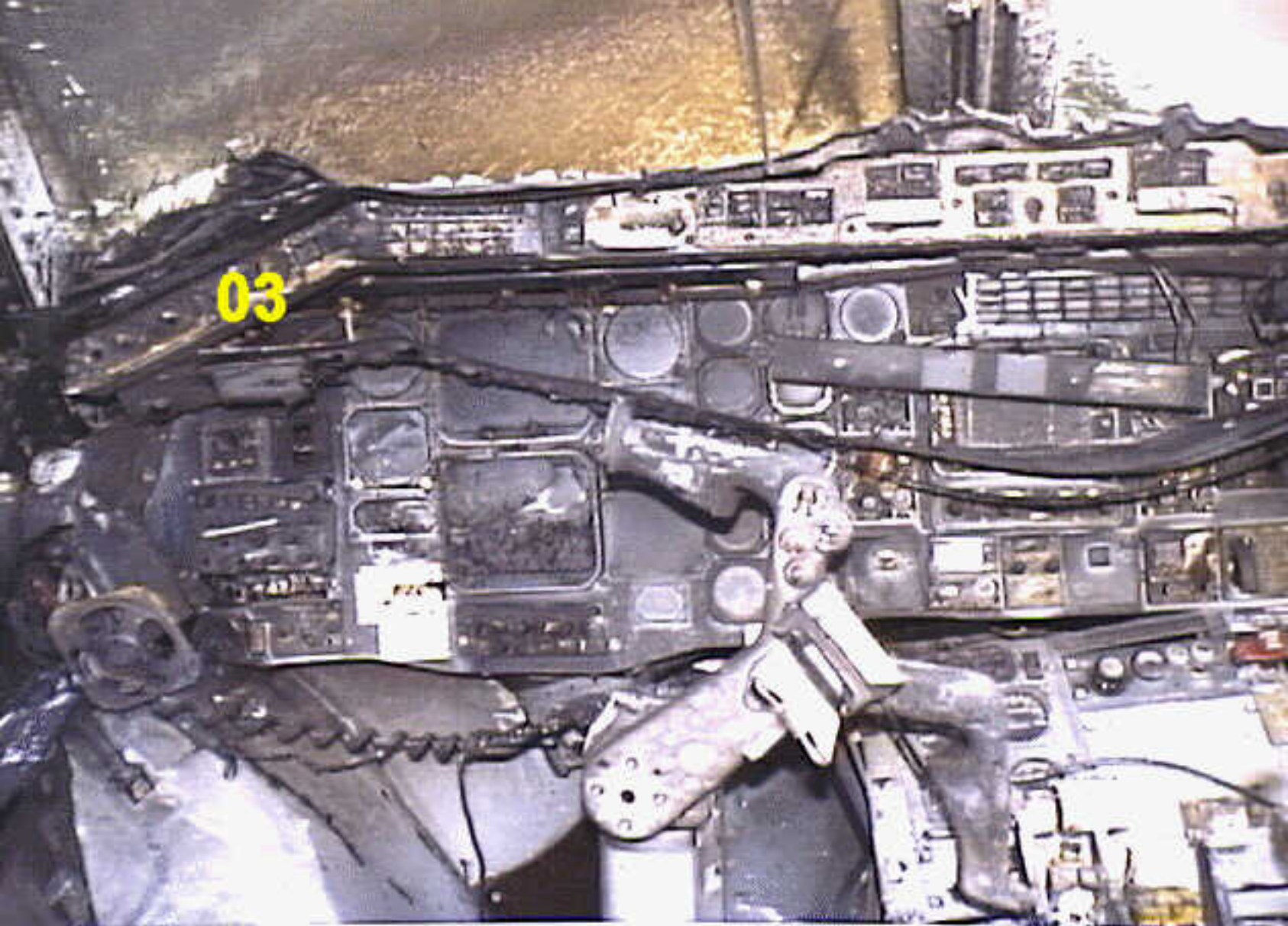
Systems 9A - Photo 03. Main Instrument Panel
