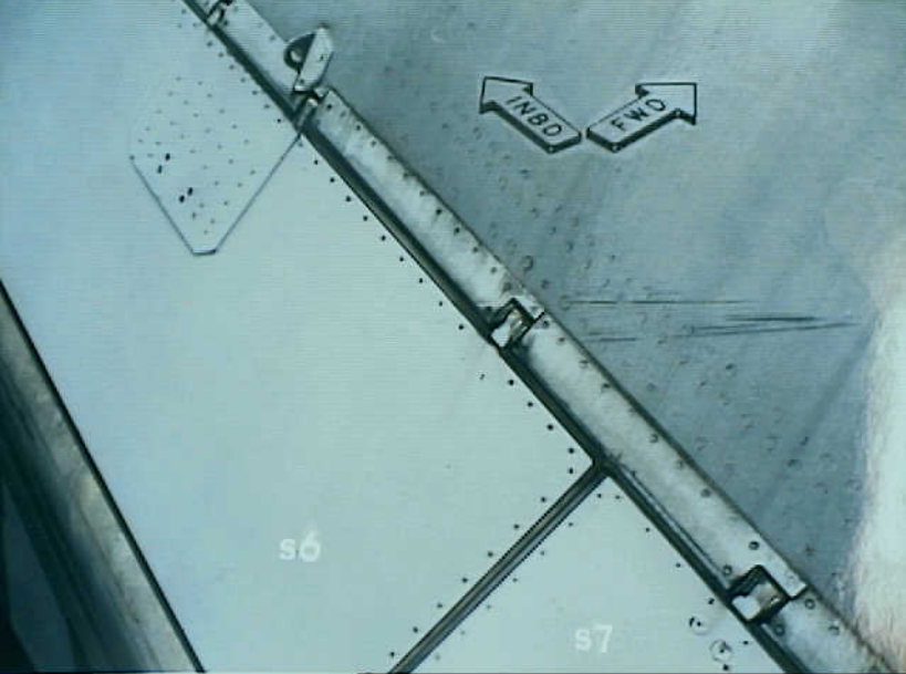
Systems 9 - Photo 8. View looking inboard of spoiler 6. Note continuous scrape pattern from wing skin onto the spoiler panel.
