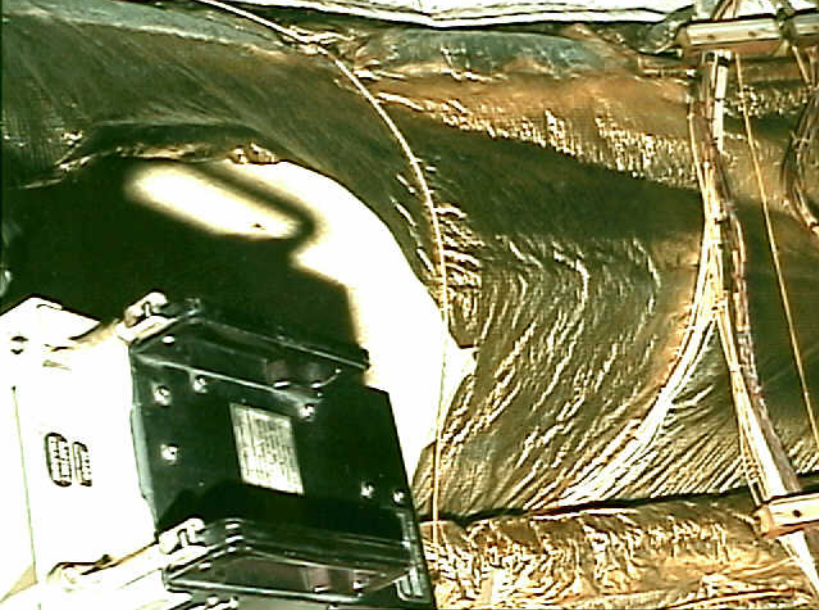
Systems 9 - Photo 8. Airplane 6. B-747(1) Aft left fuselage insulation blankets stretch wires between clamps. (2) Wire seen between foam and nylon side of raceway clamp at top left. (View is overhead. Right edge of photo is top).
