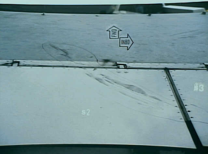
Systems 9 - Photo 7. View looking forward of spoilers 2 and 3. Note continuous scrape pattern from upper wing skin across both spoiler panels.
