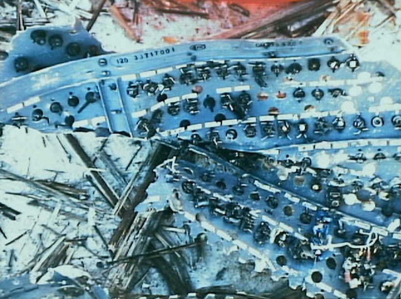
Systems 9 - Photo 6. Circuit Breaker Panel
