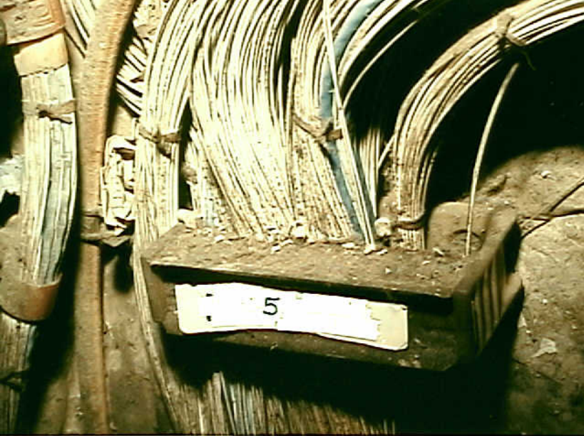
Systems 9 - Photo 6. Airplane 5. A-300 electrical compartment beneath cockpit. Wires in clamp shown with rivet fragments and drill shavings. Also visible are lint and wadded paper.
