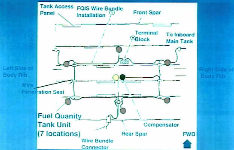
Systems 9 - Photo 56. CWT Fuel Quantity Indicator System Schematic.
