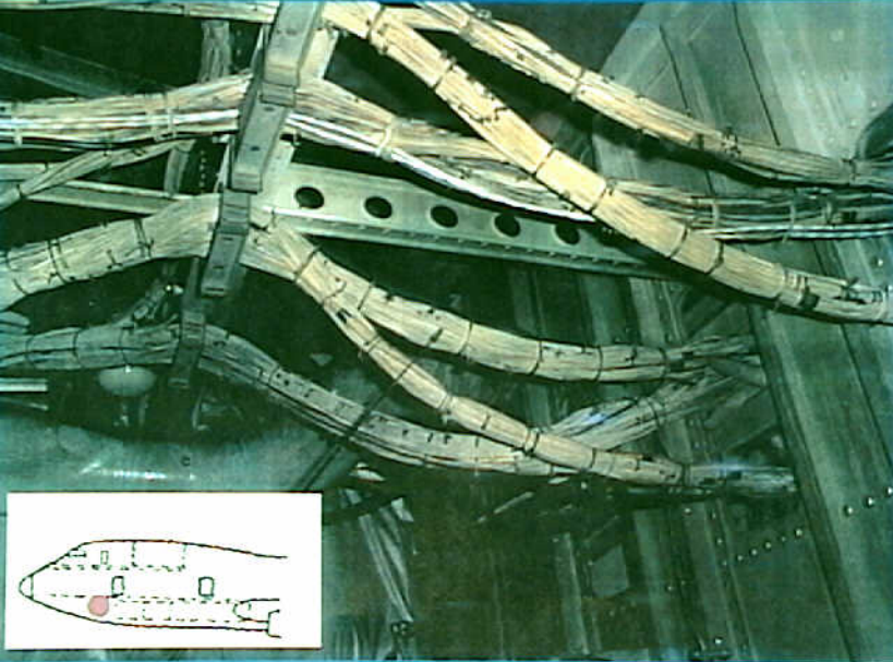
Systems 9 - Photo 53. (Feb. 21-25,1998) Pointer indicates CWT Compensator Signal Wire to Volumetric Shut-Off Unit in 3 1/4 inch diameter bundle with other
