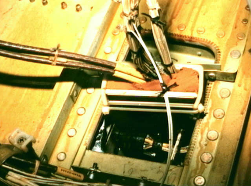
Systems 9 - Photo 51. (Feb. 21-25, 1998) B-747 opening and wire behind bundle at left of photo 50. Clamp sprung open when plastic panduit (ty-wrap) was removed. Visible are degraded foam, brown on wires, and power cables routed with system wires.
