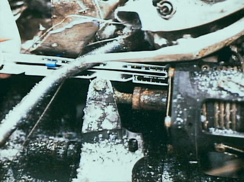
Systems 9 - Photo 5. Measurement of Rudder Trim Spool Rod Extension
