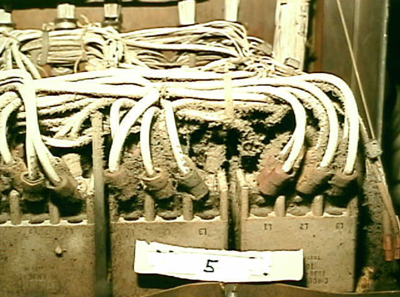
Systems 9 - Photo 5. Airplane 5. Lint bridging circuit breakers in Airbus A-300 cockpit.
