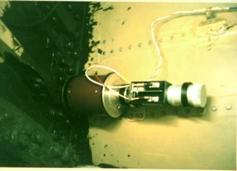
Systems 9 - Photo 47. Airplane 19. B-757 Compensator and wire insulation. Roughened wire insulation was found where wires contacted the corners of the can shaped lower portion and near the row of rivets. (Top of compensator shown to right).
