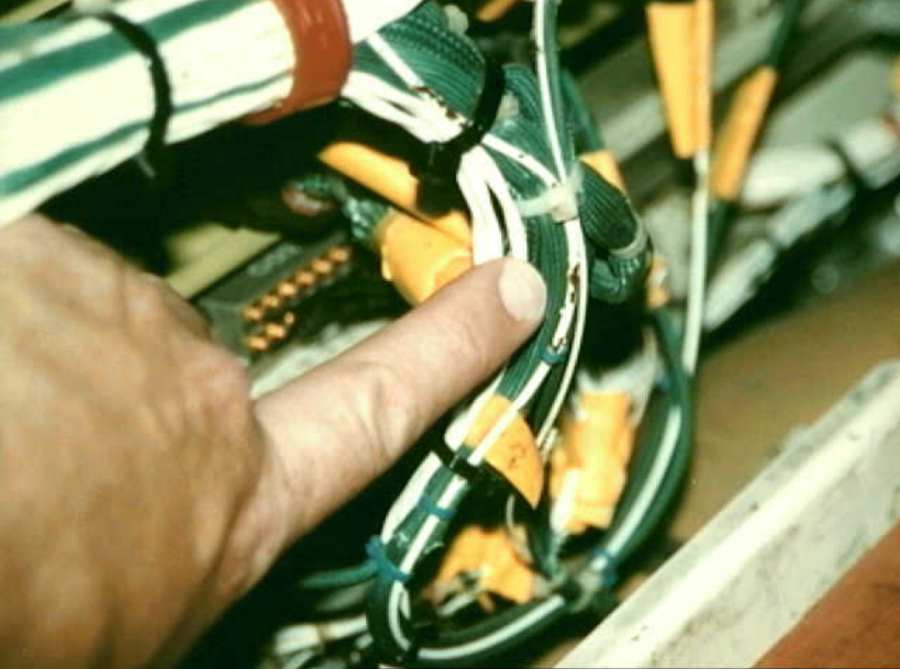
Systems 9 - Photo 46. Airplane 21. B-757 wires found mechanically damaged in electronic/equipment compartment, behind avionics rack.
