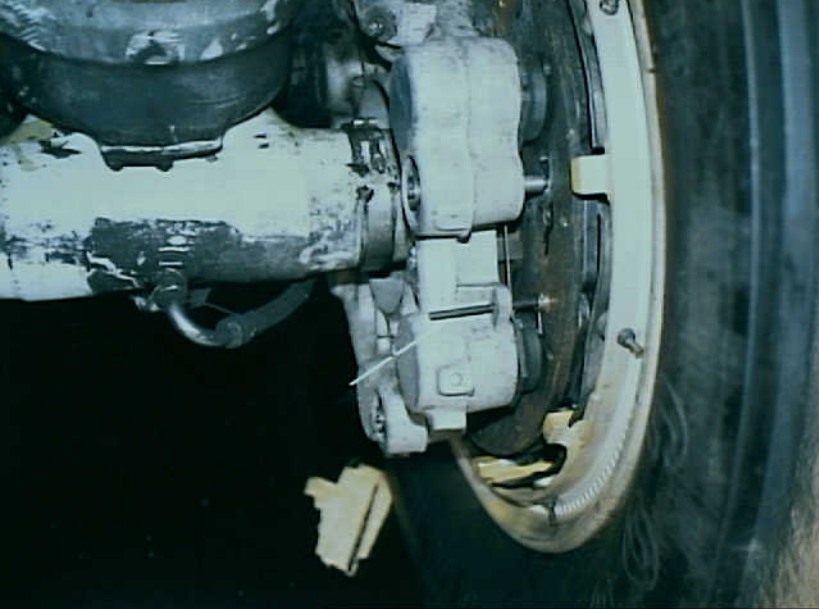
Systems 9 - Photo 4. View of looking forward of the right outboard brake assembly. Note the length of the wear pin (unpressurized).
