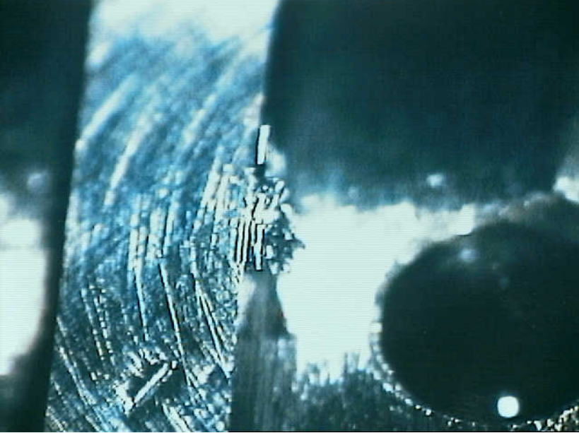
Systems 9 - Photo 4. Sheared at 53 lbs. Test 3 - Photo A Chip in Place
