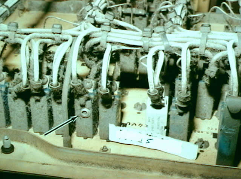
Systems 9 - Photo 4. Airplane 5. Hardware (washer) on circuit breaker and lint accumulation. Location is inside of opened circuit breaker panel in Airbus A-300 cockpit.
