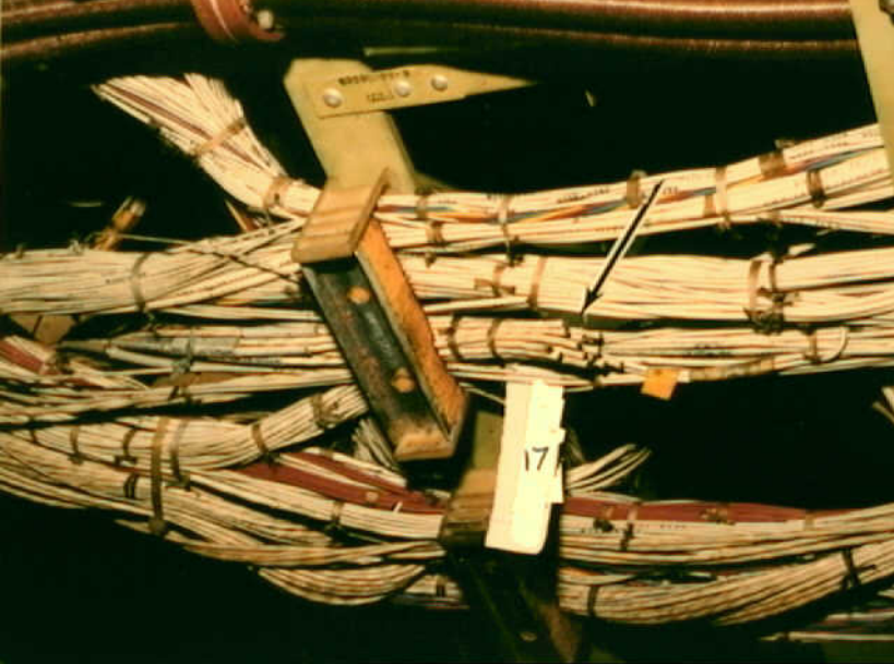
Systems 9 - Photo 39. Airplane 17. B-747 wire bundle cut off above forward cargo compartment. (Cargo liner removed for visibility).
