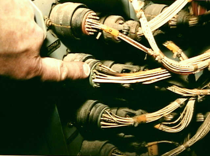
Systems 9 - Photo 36. Airplane 16. B-747 wire insulation outboard of (P6) circuit breaker panel is split and dark brown where it comes from the connector. Copper conductor is visible. Note plug missing two holes
