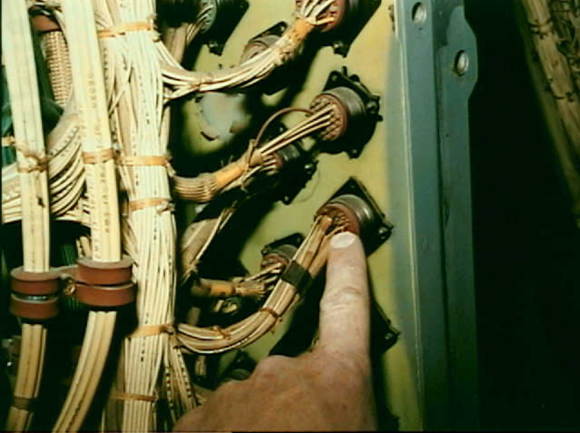
Systems 9 - Photo 35. Airplane 16. B-747 wire insulation in (P6) circuit breaker panel is dark brown where it comes from the connector and enters woven sleeve (wire at top of connector).
