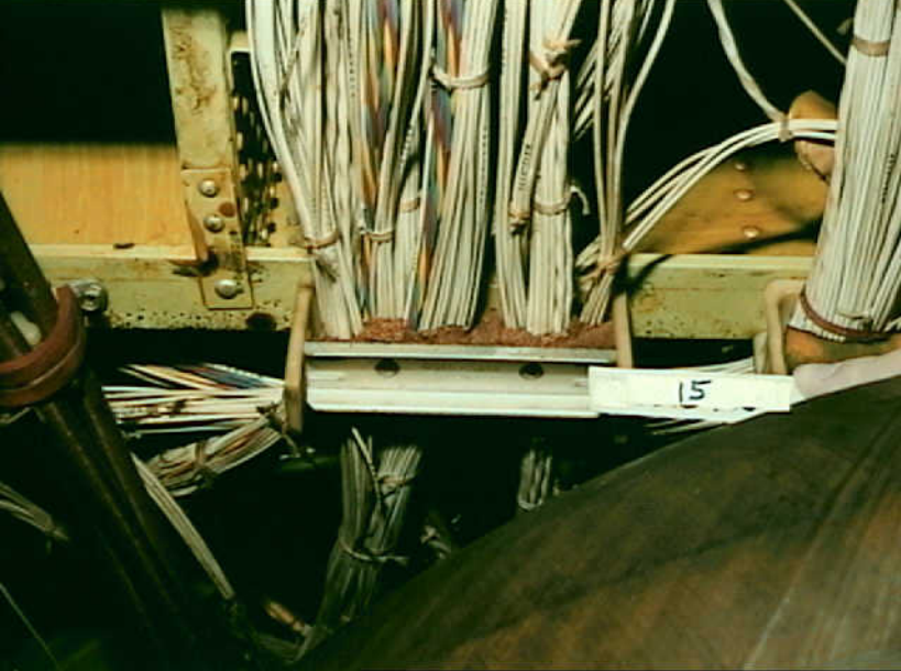
Systems 9 - Photo 34. Airplane 15. B747 degraded foam in raceway clamp above potable water bottle. Wires on hardened adhesive. Blue fluid on clamp to right and along bottom of floor beam. Brown corrosion inhibitor is visible. Paper fragment on wire.
