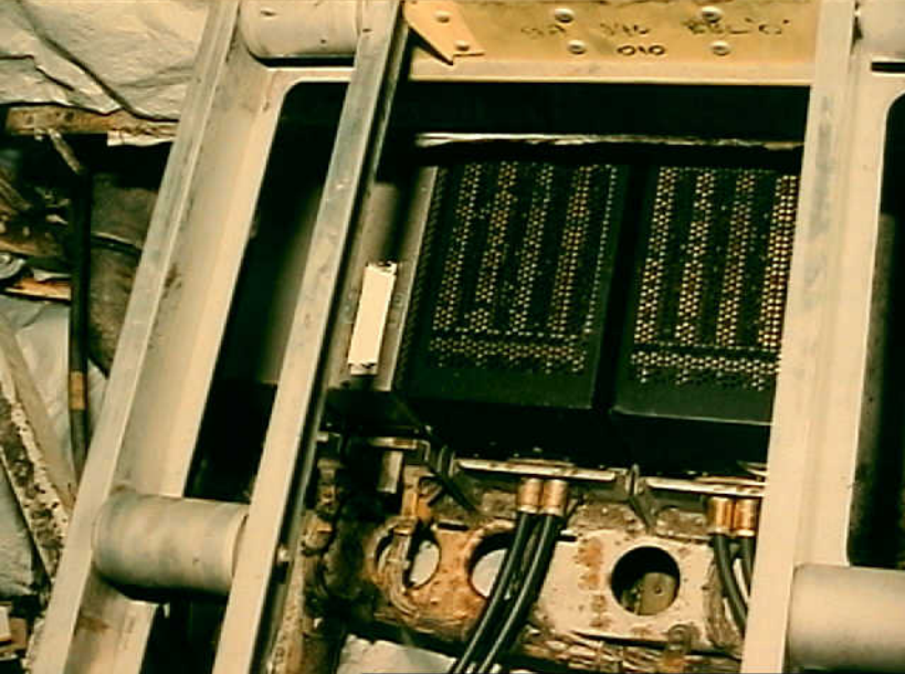
Systems 9 - Photo 33. Airplane 15. B-747 avionics visible beneath forward cargo compartment. Metal shavings are on black boxes near open holes that expose internal circuits and components. (View is down. Top of photo is forward).
