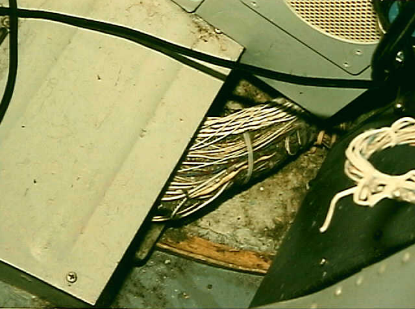
Systems 9 - Photo 32. Airplane 14. B-747 cockpit floor aft and outboard of First Officer seat. Wire bundle was stiff and not flexible, containing bared wire fragments, metal shavings, dirt, and a mixture of wire types. New wires laid on existing bundle.
