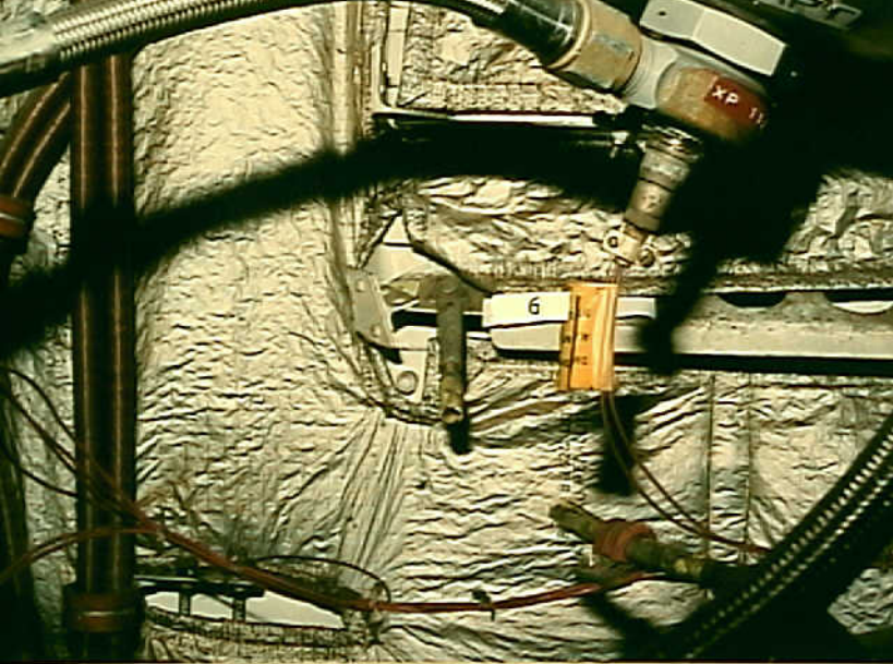
Systems 9 - Photo 31. Airplane 13. B-747 forward spar, right side. Broken fire extinguisher bracket visible.
