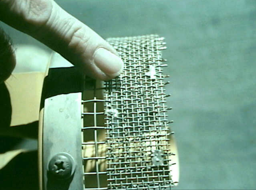
Systems 9 - Photo 26. Airplane 12. Wire curl found in B-747 scavenge pump inlet screen. (Bottom of screen at right in photo).
