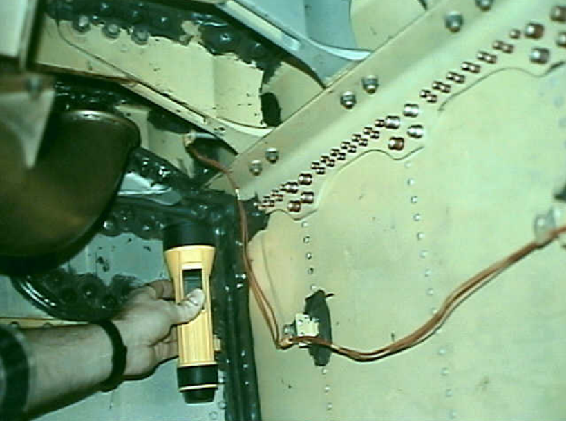
Systems 9 - Photo 25. Airplane 12. B-747 in CWT, showing CWT FQIS wire chafe on structure.
