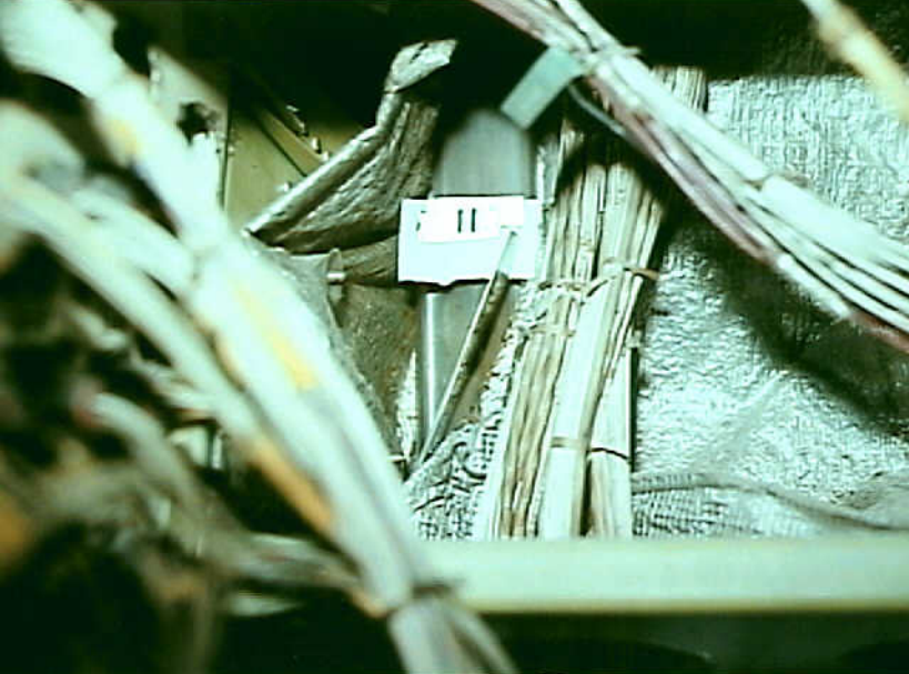
Systems 9 - Photo 23. Airplane 11. B-747 above left wing/fuselage pressure seals near forward spar. Dinner knife (blade is upward) found next to wiring had a Pan American Airlines logo. The airplane was owned by a cargo airline when retired from service.
