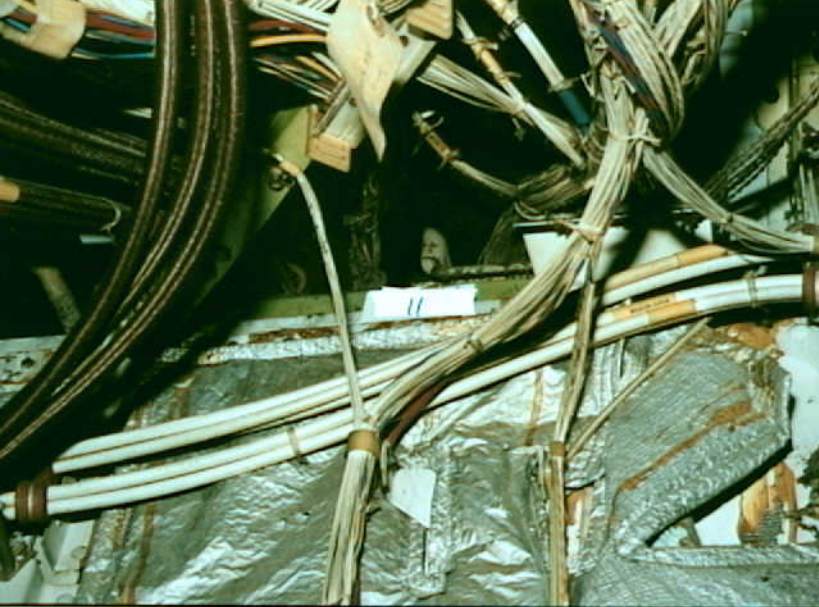
Systems 9 - Photo 21. Airplane 11. B-747 at top left of forward spar, looking aft. Visible are lint, torn insulation, and wire bundles stretched between clamps.
