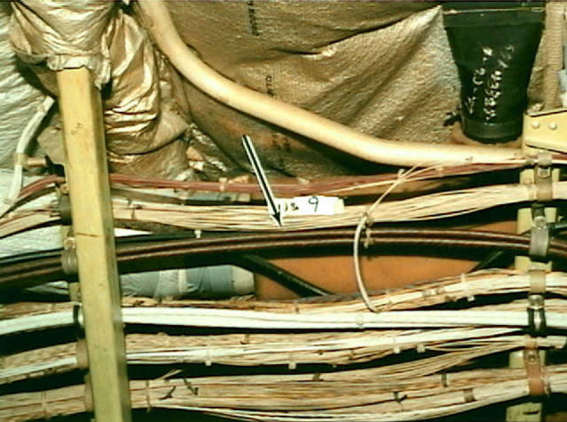
Systems 9 - Photo 20. Airplane 9. B-747 wire installation forward of photo 19 shows CWT FQIS wires in W480 sag and rub galley power cable. Splices are half exposed in clamp at upper left, behind structure (beneath red wires). Capped wire is at right.
